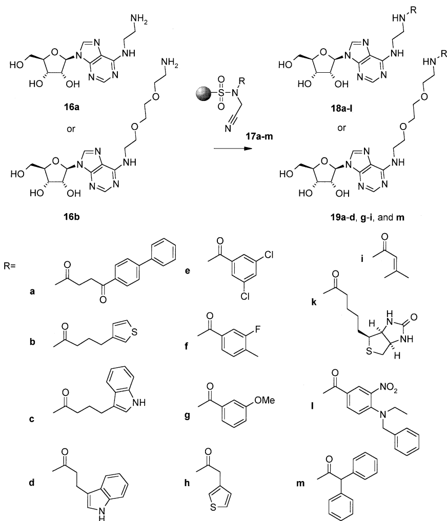
Scheme 5. Polymer-assisted synthesis of N^6 -substituted adenosine derivatives 18a–l and 19a–d, g–i, and m .
