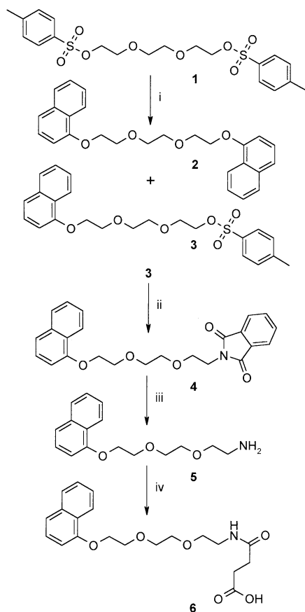
Scheme 1. Synthesis of 2-[2-(2-Naphthyl-1-yloxy-ethoxy)-ethoxy]-ethylamine ( 5 ) and succinamic acid derivative 6 : (i): 1-naphthol, NaH, THF, reflux; (ii) phthalimide potassium, DMF, 90 °C; (iii) hydrazine hydrate, EtOH, reflux; (iv) succinic anhydride, Et 3 N, Na 2 CO 3 , CH 2 Cl 2 .
