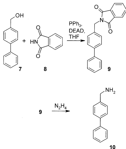
Scheme 2. Synthesis of 4-phenyl-benzyl amine ( 10 ) from 4-phenyl-benzyl alcohol ( 7 ).
